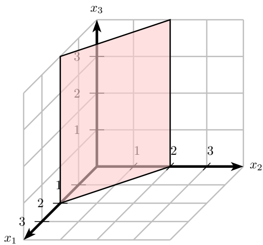
Abb. 3: E_5 : x_1 + x_2 = 2
